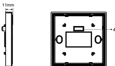
Figure 8. Dimensions - Side View Figure 9. Components - Back View
