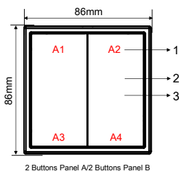
Figure 7. Dimensions - Plastic version
