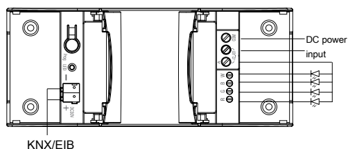
Figure 6. Wiring
